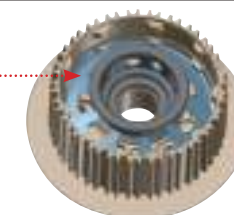
disco spingimolla primaria spring pusher plate
